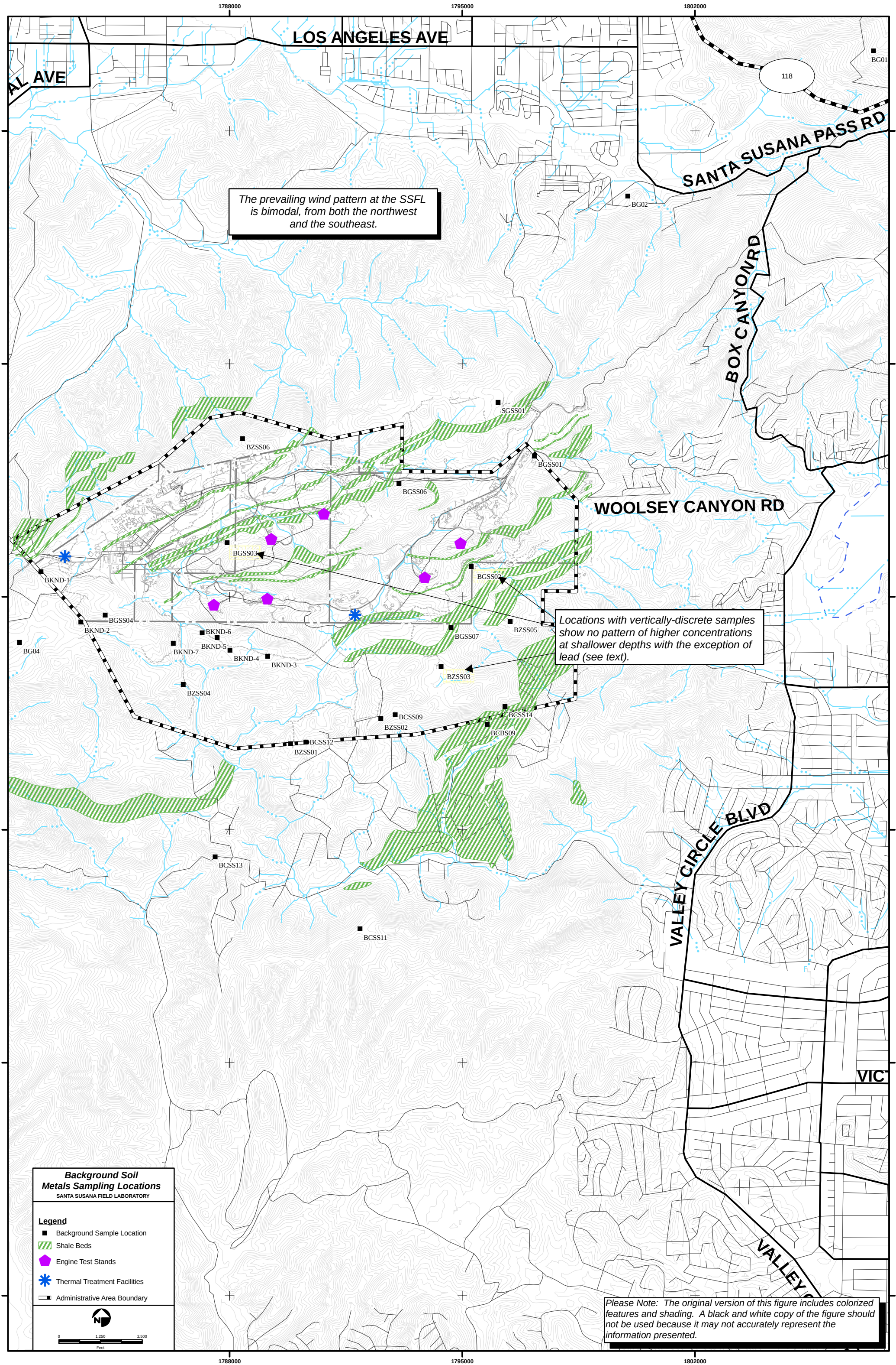
Vertical Distribution of Metals in Sampling Results SSFL Soil Background
